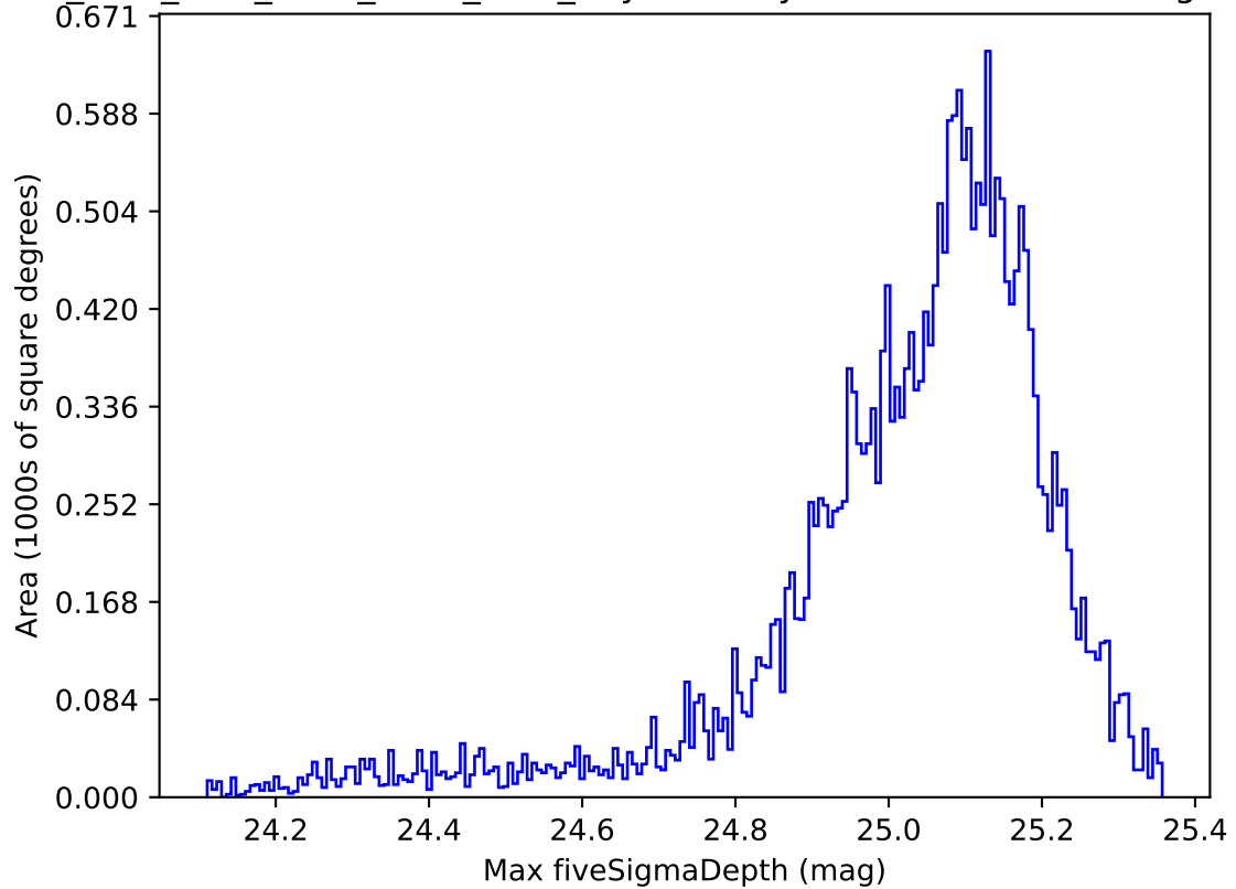
ddf_acor_sf15_lsf40_lsr20_v3.4_10yrs All sky all bands: Max fiveSigmaDepth
