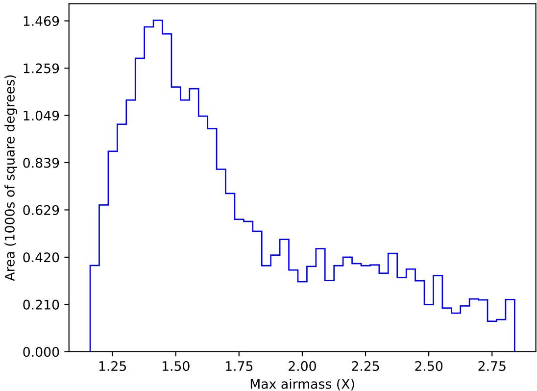
ddf_acor_sf15_lsf40_lsr20_v3.4_10yrs Yr 1 z band: Max airmass
