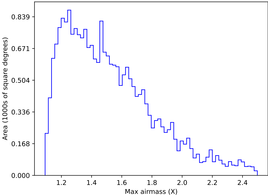
ddf_acor_sf15_lsf40_lsr20_v3.4_10yrs Yr 1 u band: Max airmass
