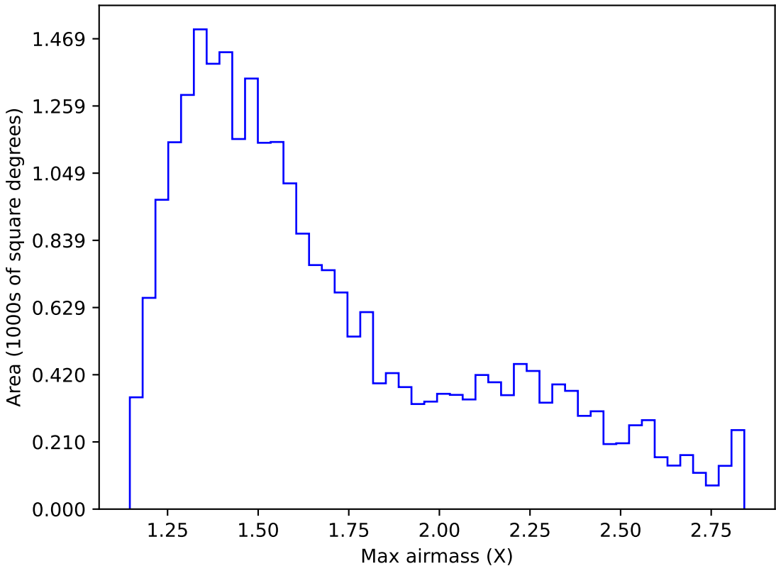
ddf_acor_sf15_lsf40_lsr20_v3.4_10yrs Yr 1 i band: Max airmass
