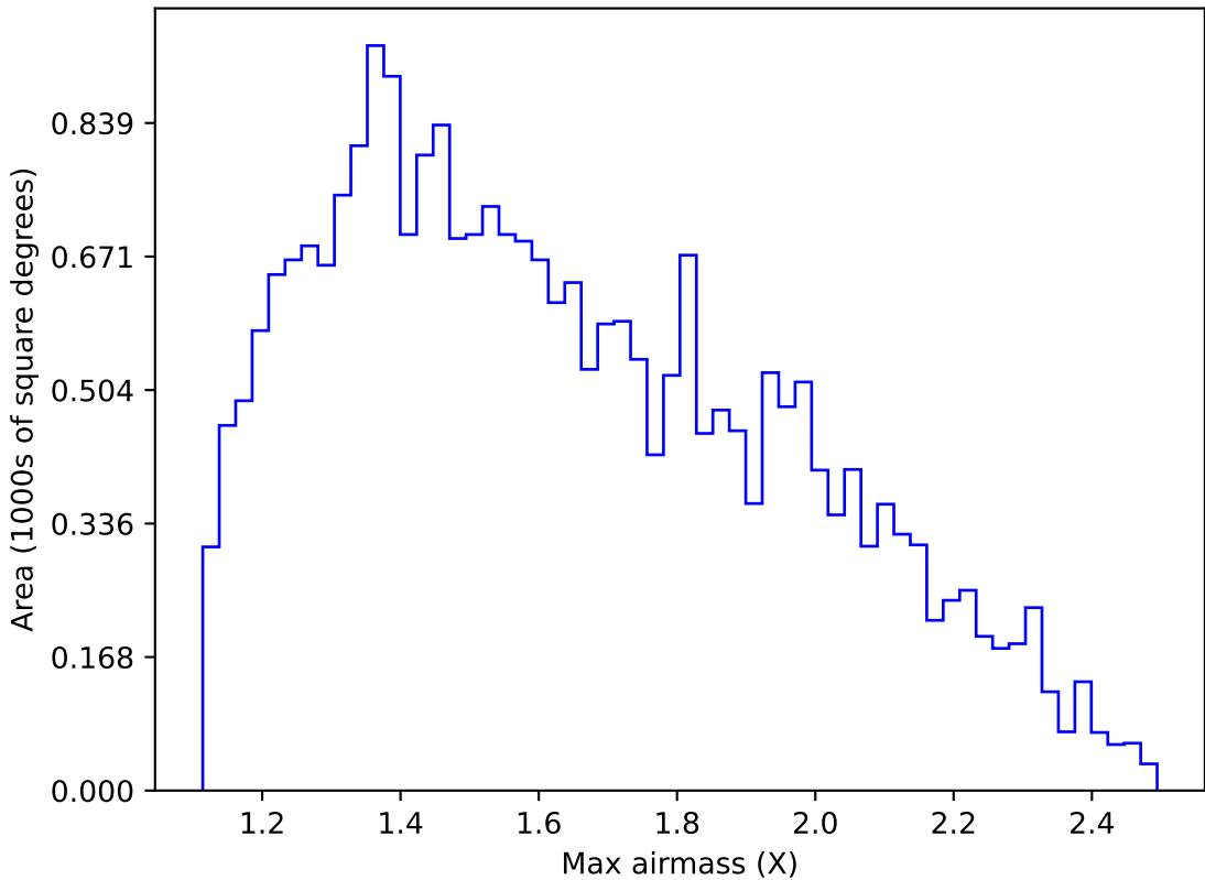
ddf_acor_sf15_lsf40_lsr20_v3.4_10yrs Yr 1 g band: Max airmass
