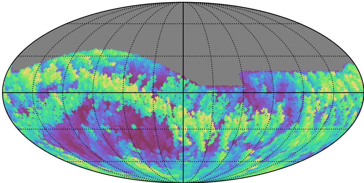
ddf_acor_sf15_lsf40_lsr20_v3.4_10yrs Yr 1 all bands: Max airmass
