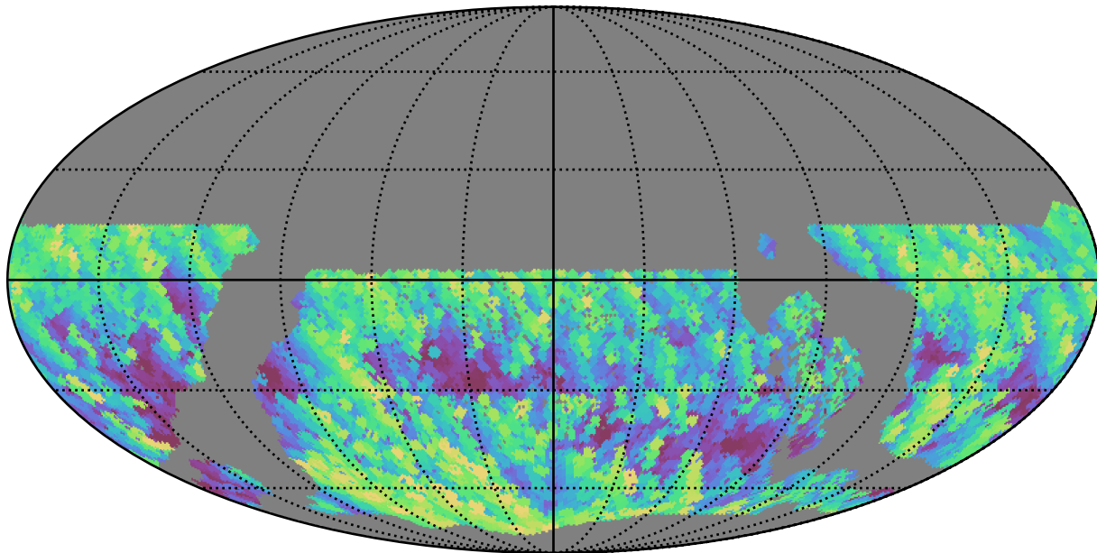
ddf_acor_sf15_lsf40_lsr20_v3.4_10yrs WFD y band: Max airmass
