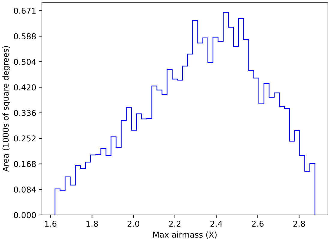
ddf_acor_sf15_ls40_lsr20_v3.4_10yrs WFD y band: Max airmass
