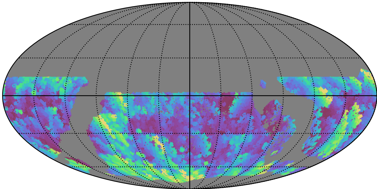
ddf_acor_sf15_lsf40_lsr20_v3.4_10yrs WFD u band: Max airmass
