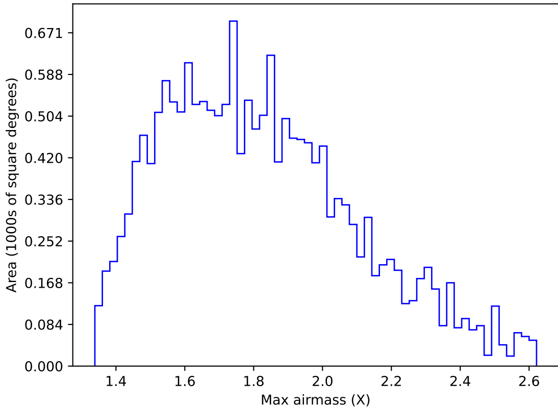
ddf_acor_sf15_ls40_lsr20_v3.4_10yrs WFD u band: Max airmass
