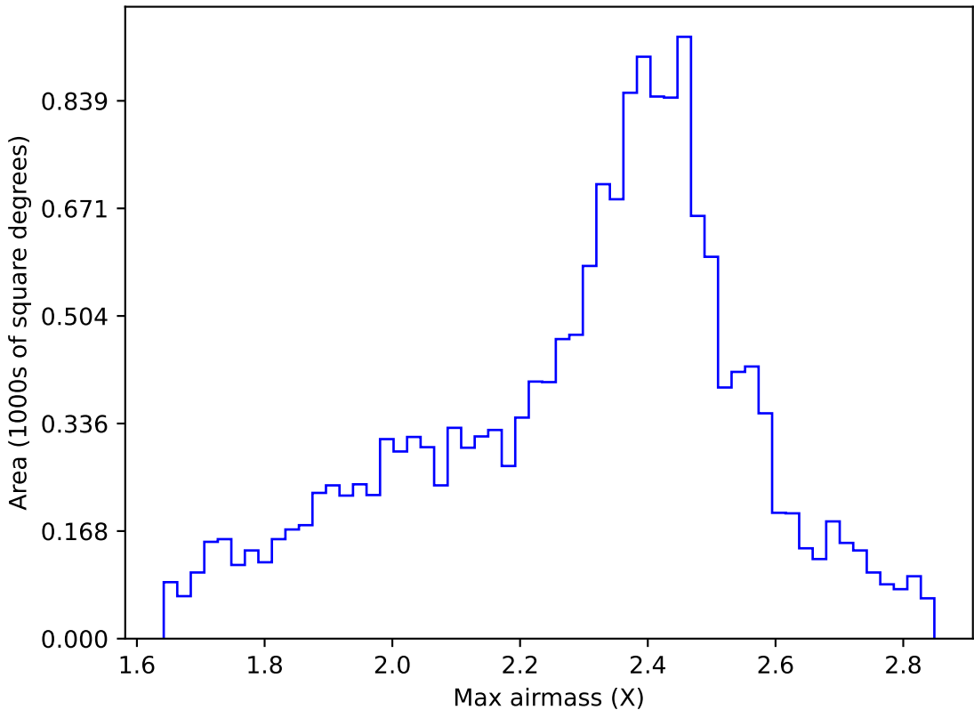
ddf_acor_sf15_lsf40_lsr20_v3.4_10yrs WFD r band: Max airmass
