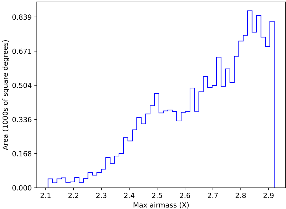
ddf_acor_sf15_lsf40_lsr20_v3.4_10yrs WFD all bands: Max airmass
