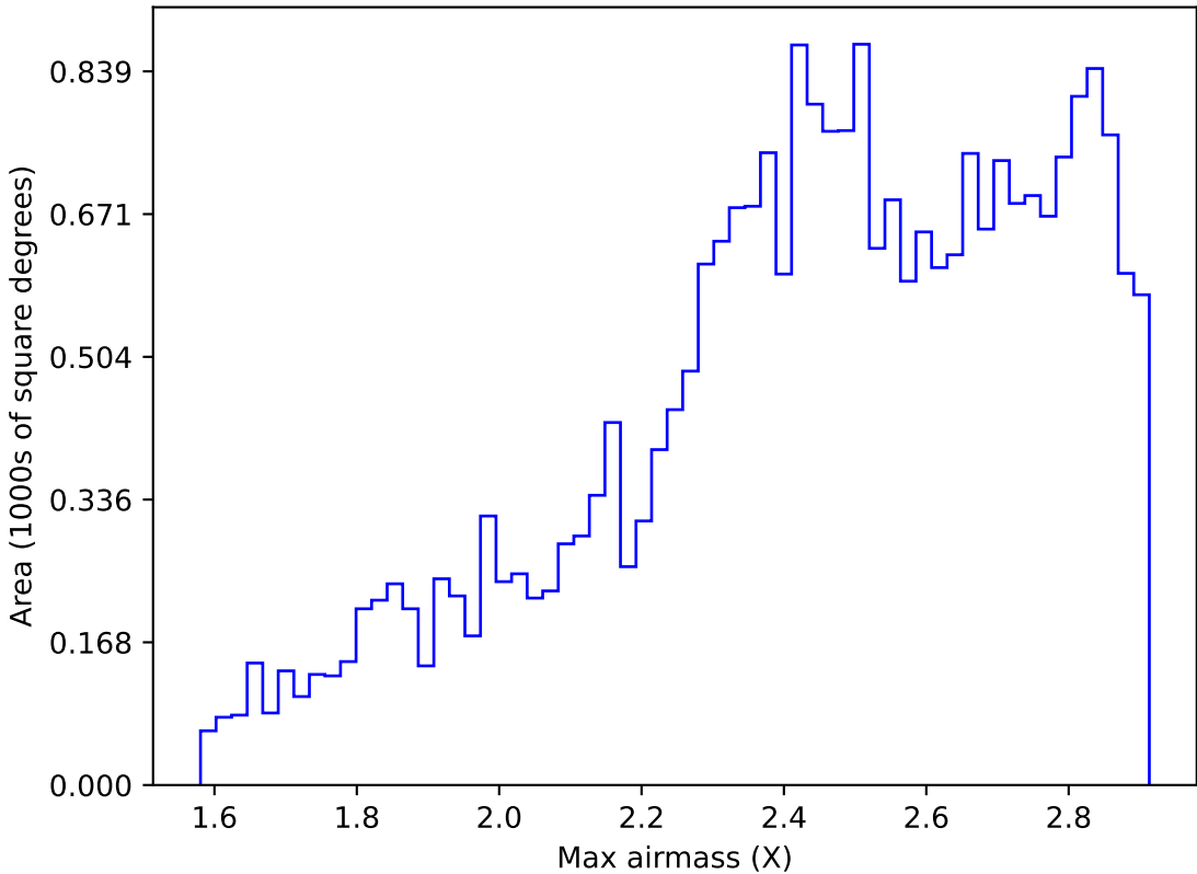
ddf_acor_sf15_lsf40_lsr20_v3.4_10yrs All sky z band: Max airmass
