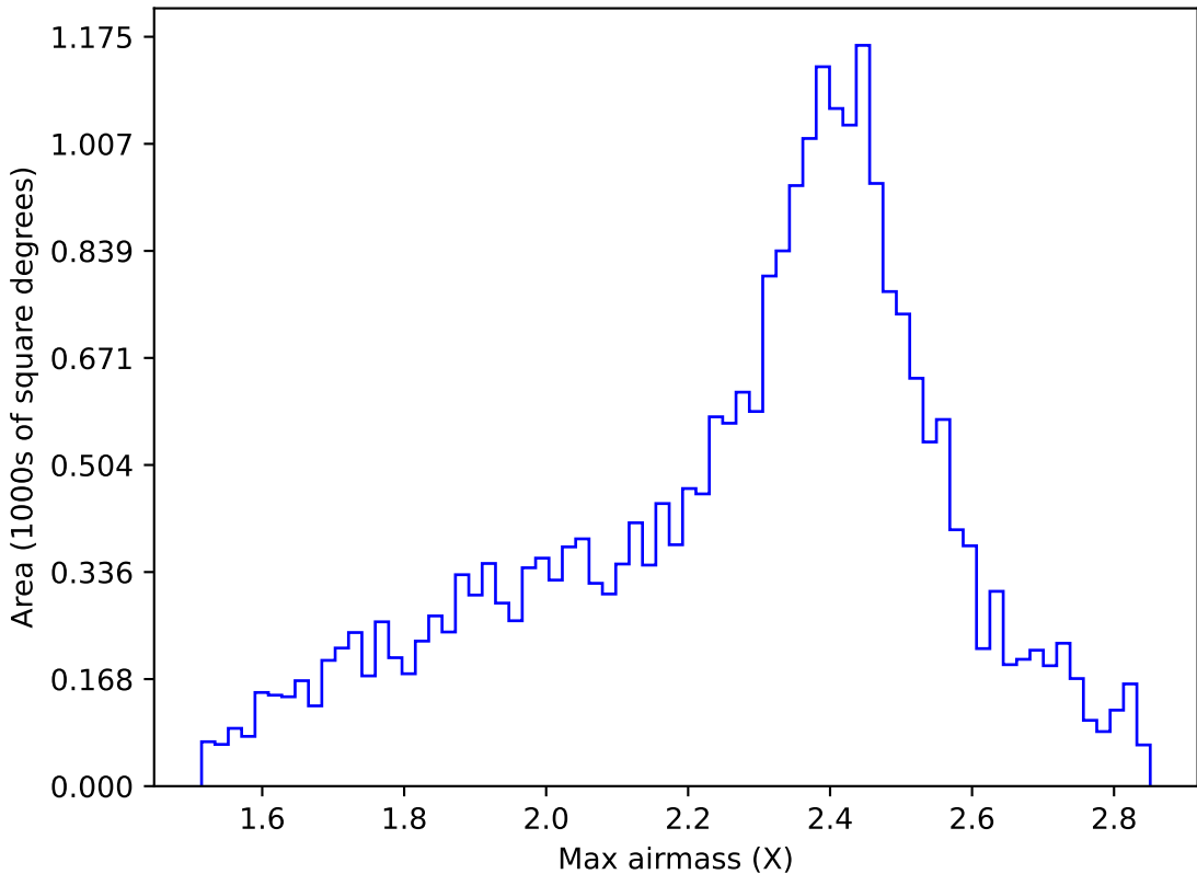
ddf_acor_sf15_lsf40_lsr20_v3.4_10yrs All sky r band: Max airmass
