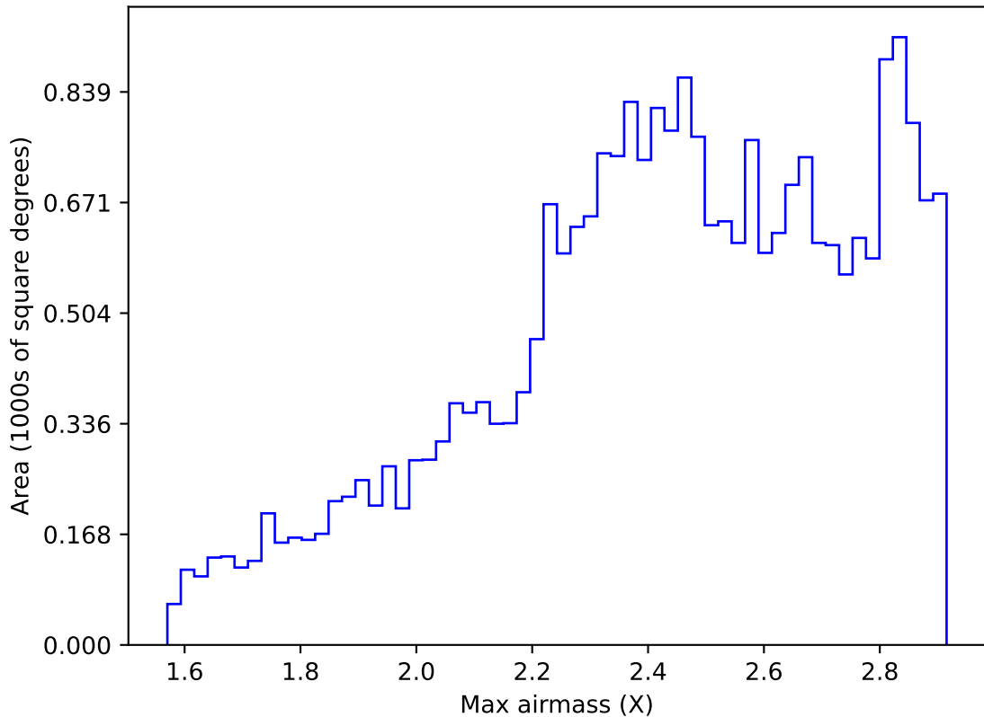
ddf_acor_sf15_lsf40_lsr20_v3.4_10yrs All sky i band: Max airmass
