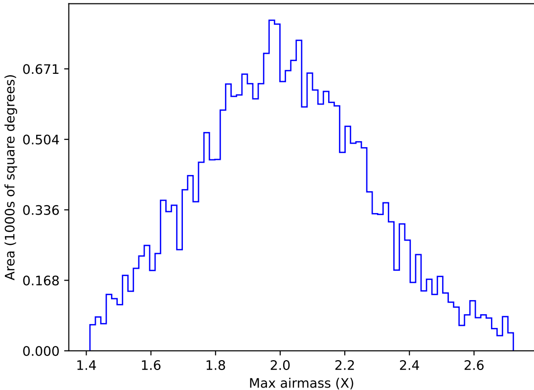
ddf_acor_sf15_lsf40_lsr20_v3.4_10yrs All sky g band: Max airmass
