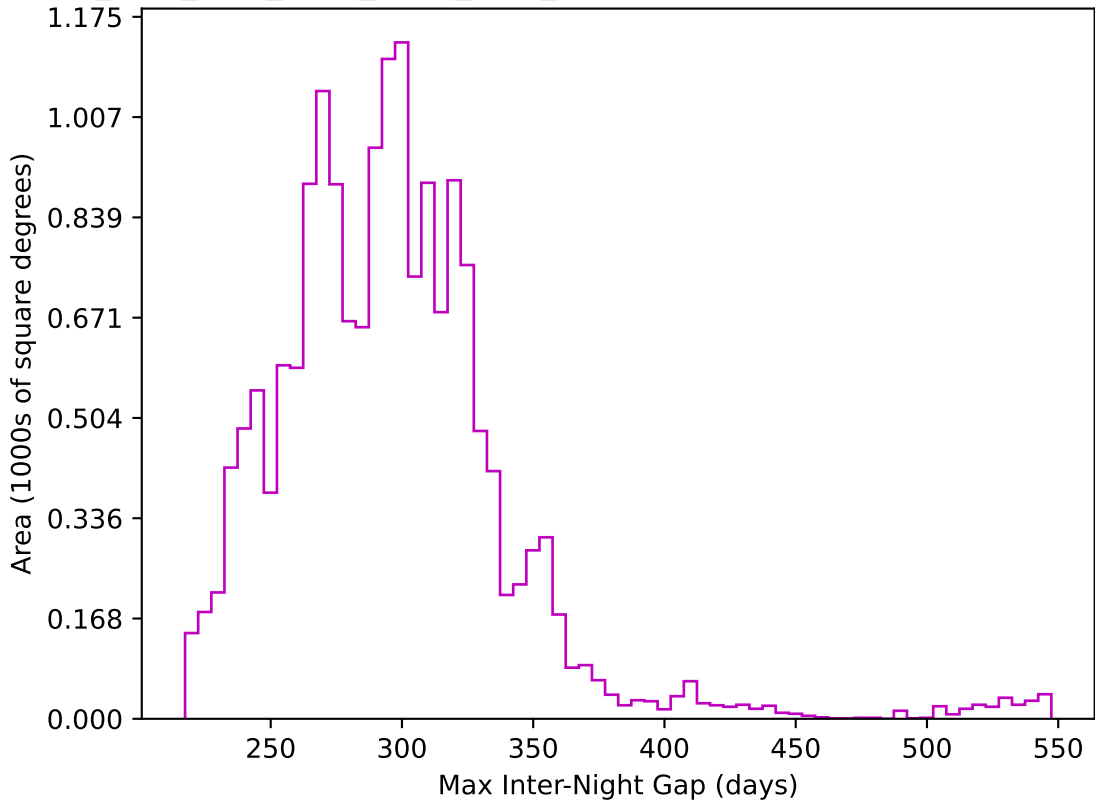
ddf_acor_sf15_lsf40_lsr20_v3.4_10yrs WFD z band: Max Inter-Night Gap
