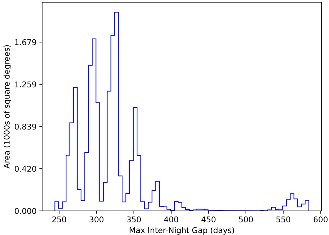
ddf_acor_sf15_lsf40_lsr20_v3.4_10yrs WFD y band: Max Inter-Night Gap
