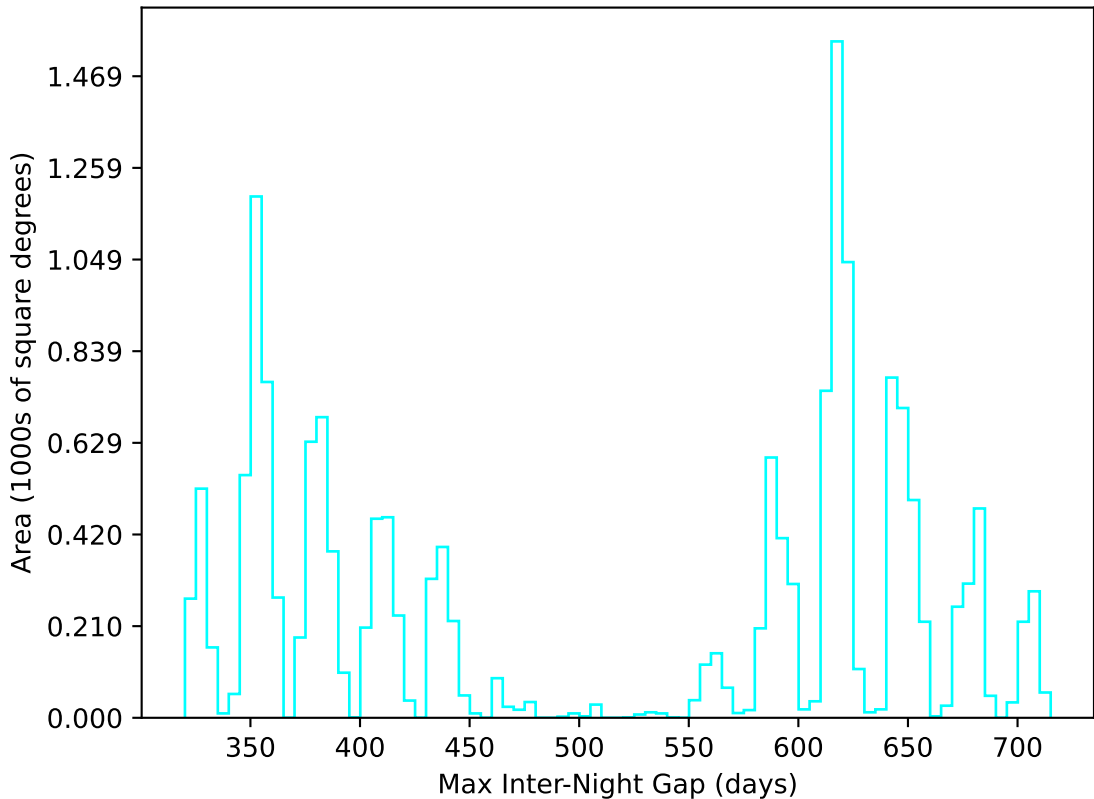
ddf_acor_sf15_lsf40_lsr20_v3.4_10yrs WFD u band: Max Inter-Night Gap
