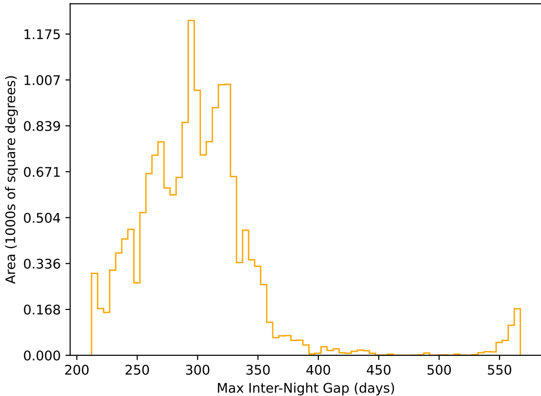
ddf_acor_sf15_lsf40_lsr20_v3.4_10yrs WFD r band: Max Inter-Night Gap
