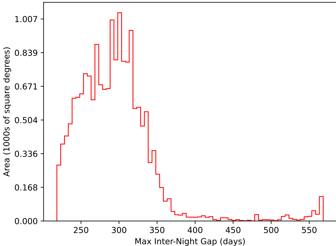
ddf_acor_sf15_lsf40_lsr20_v3.4_10yrs WFD i band: Max Inter-Night Gap
