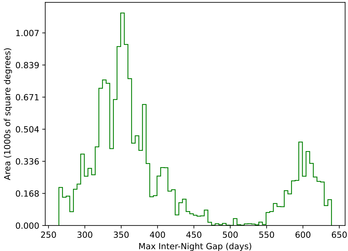
ddf_acor_sf15_lsf40_lsr20_v3.4_10yrs WFD g band: Max Inter-Night Gap
