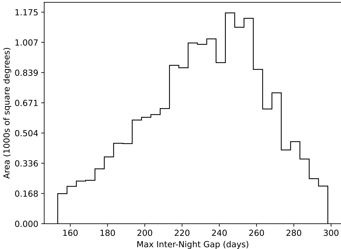
ddf_acor_sf15_lsf40_lsr20_v3.4_10yrs WFD all bands: Max Inter-Night Gap
