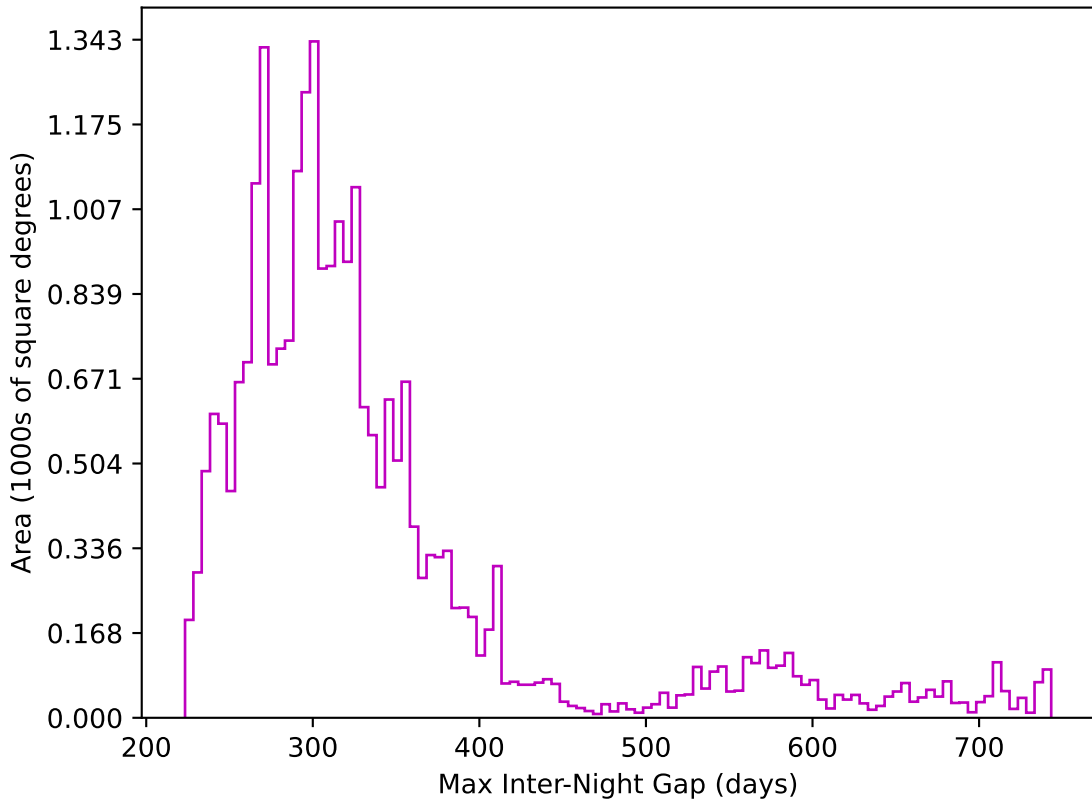
ddf_acor_sf15_lsf40_lsr20_v3.4_10yrs All sky z band: Max Inter-Night Gap
