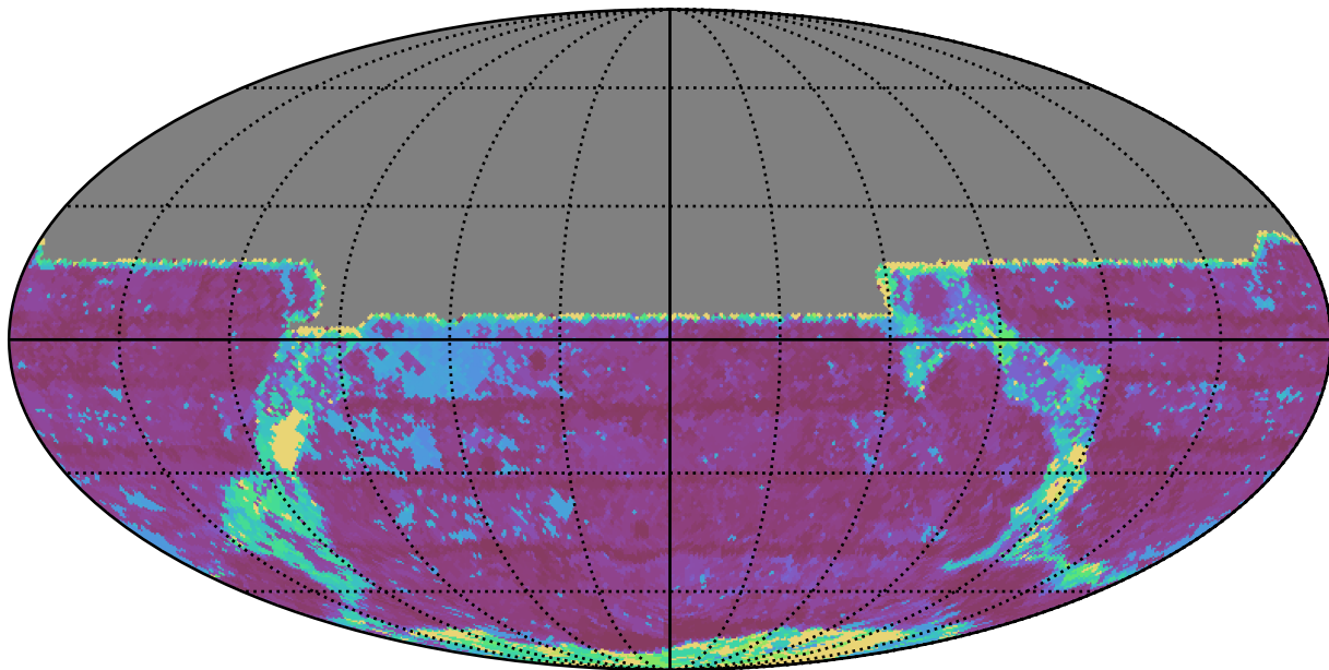
ddf_acor_sf15_lsf40_lsr20_v3.4_10yrs All sky y band: Max Inter-Night Gap
