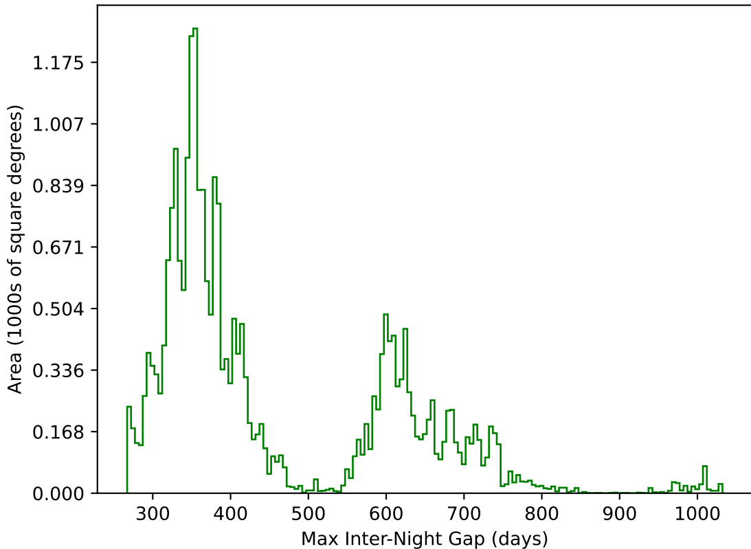
ddf_acor_sf15_lsf40_lsr20_v3.4_10yrs All sky g band: Max Inter-Night Gap
