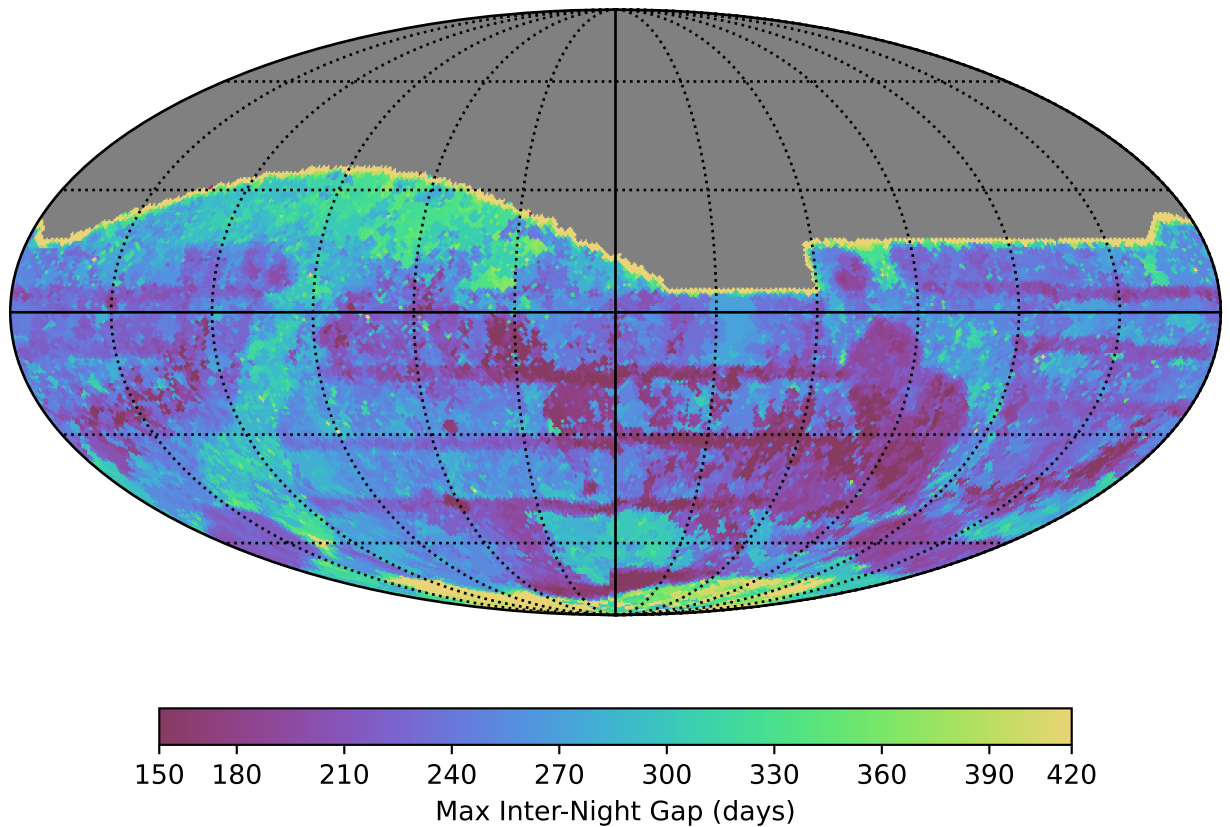
ddf_acor_sf15_lsf40_lsr20_v3.4_10yrs All sky all bands: Max Inter-Night Gap
