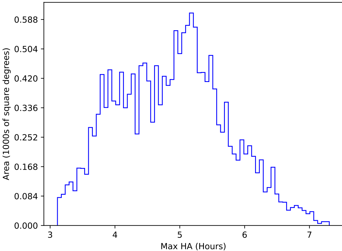
ddf_acor_sf15_lsf40_lsr20_v3.4_10yrs WFD i band: Max HA
