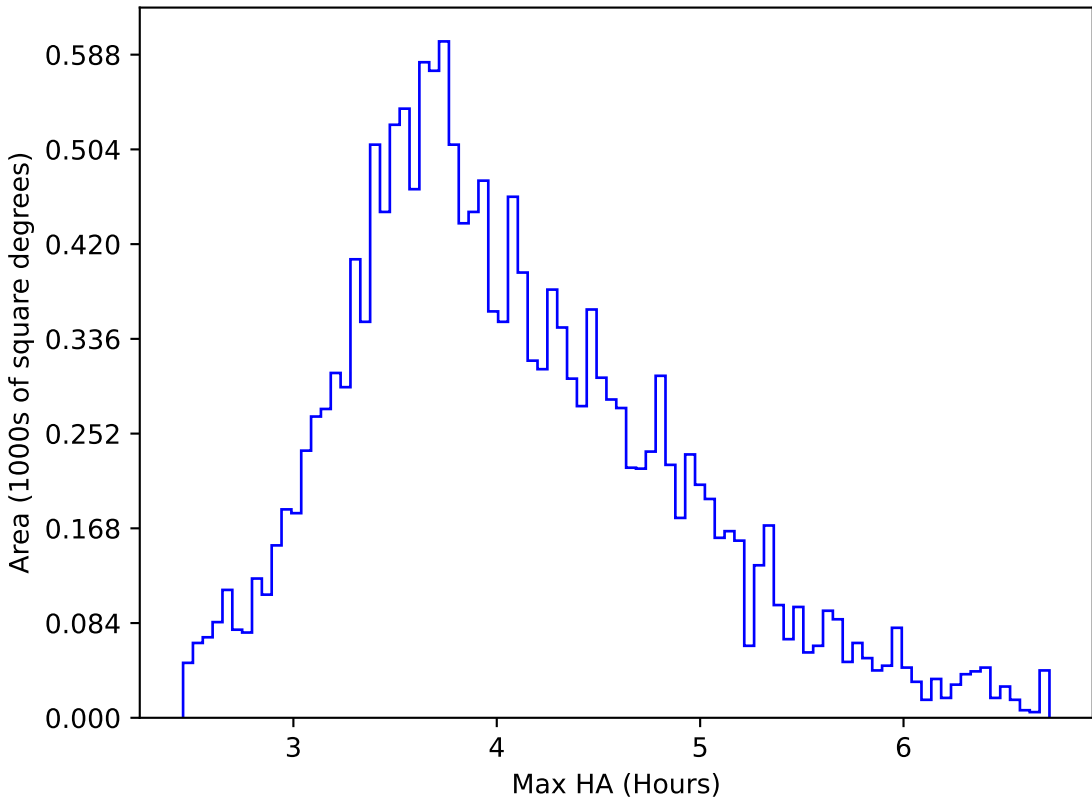
ddf_acor_sf15_lsf40_lsr20_v3.4_10yrs WFD g band: Max HA
