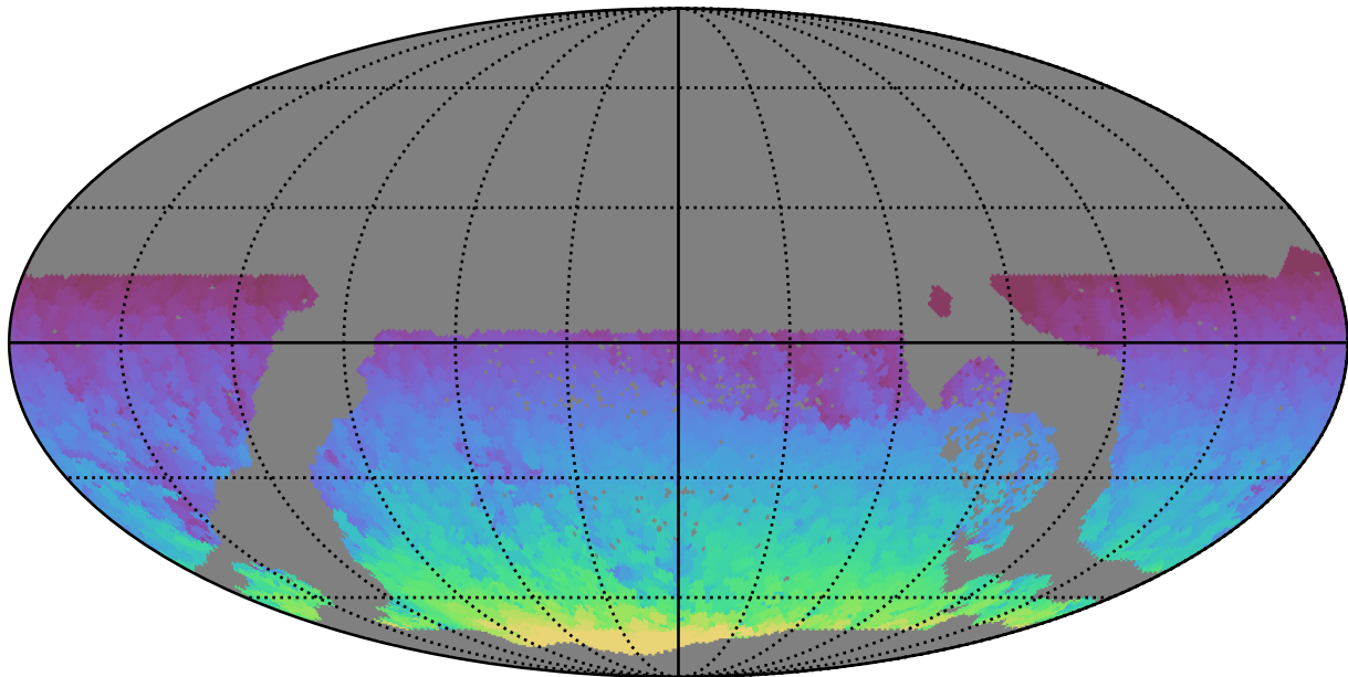
ddf_acor_sf15_lsf40_lsr20_v3.4_10yrs WFD all bands: Max HA
