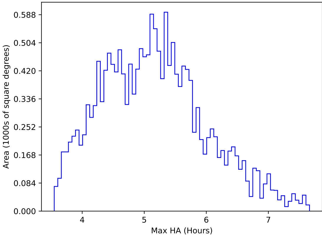
ddf_acor_sf15_lsf40_lsr20_v3.4_10yrs WFD all bands: Max HA
