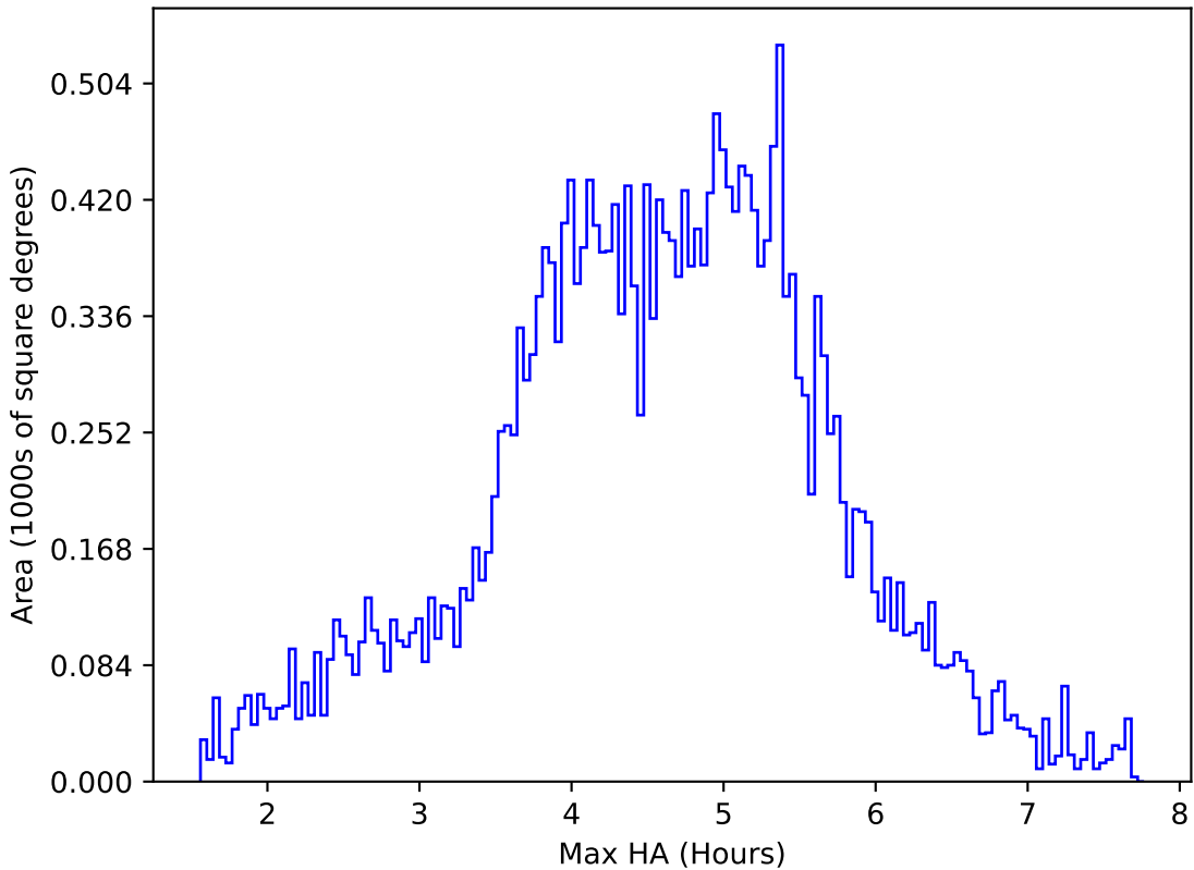
ddf_acor_sf15_lsf40_lsr20_v3.4_10yrs All sky z band: Max HA
