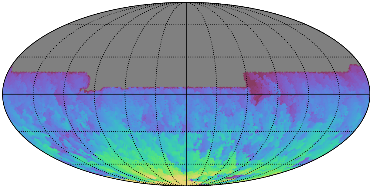
ddf_acor_sf15_lsf40_lsr20_v3.4_10yrs All sky y band: Max HA
