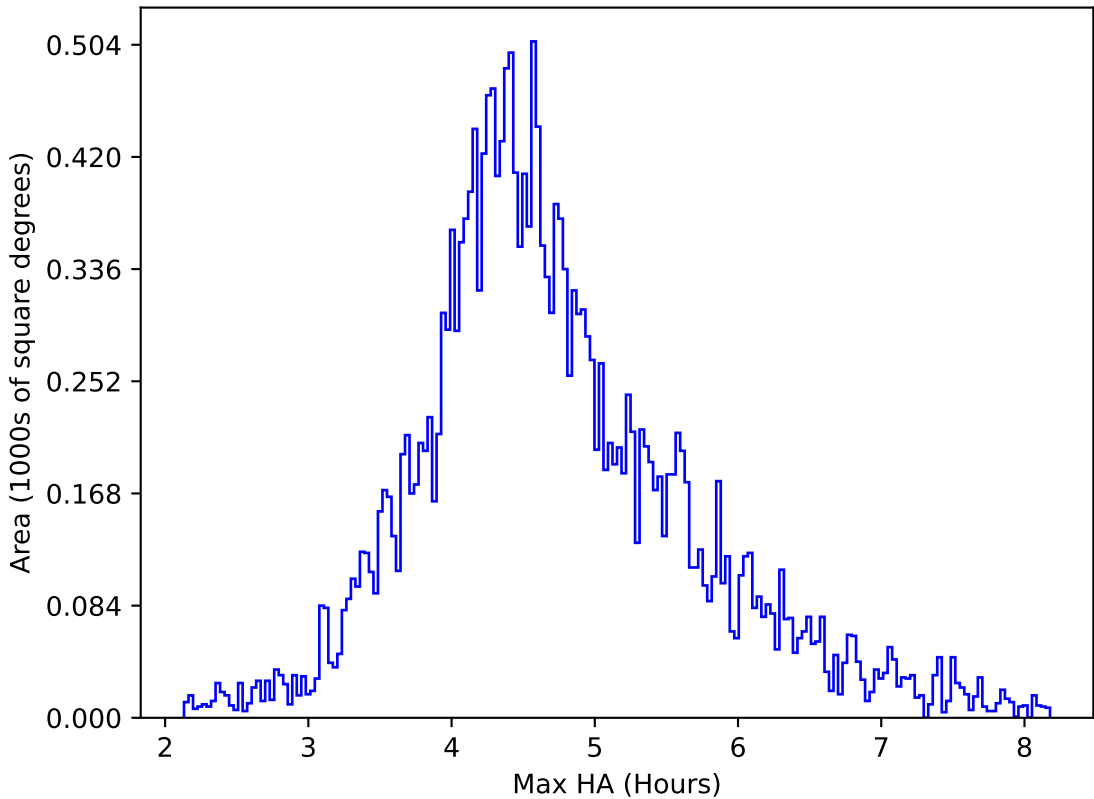
ddf_acor_sf15_ls40_lsr20_v3.4_10yrs All sky y band: Max HA
