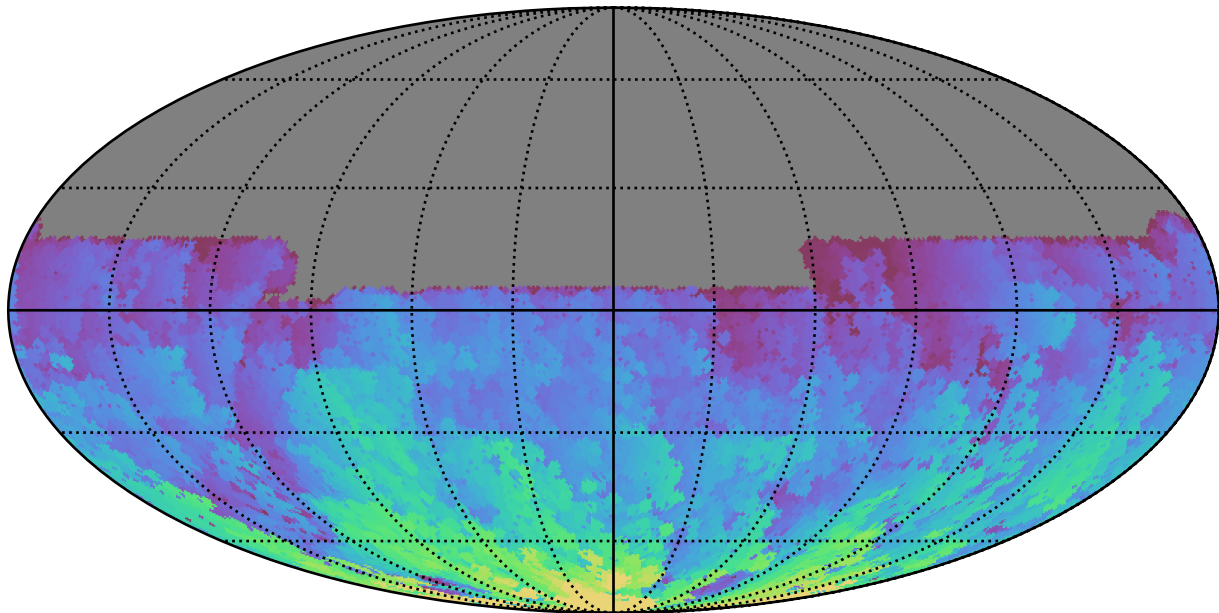
ddf_acor_sf15_lsf40_lsr20_v3.4_10yrs All sky u band: Max HA
