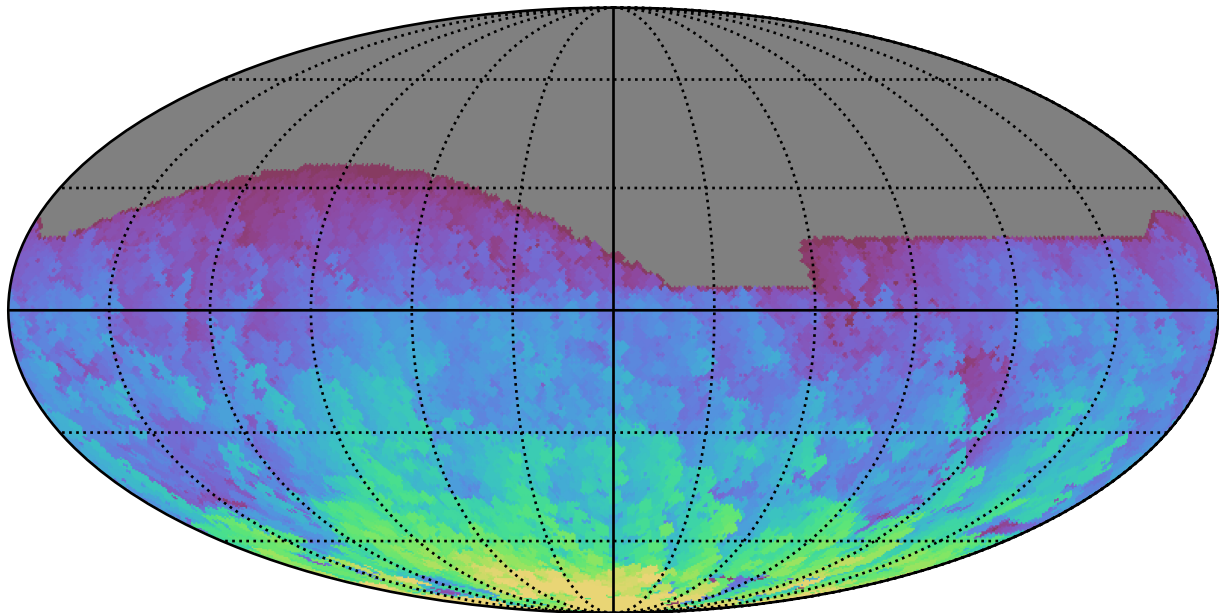
ddf_acor_sf15_lsf40_lsr20_v3.4_10yrs All sky r band: Max HA
