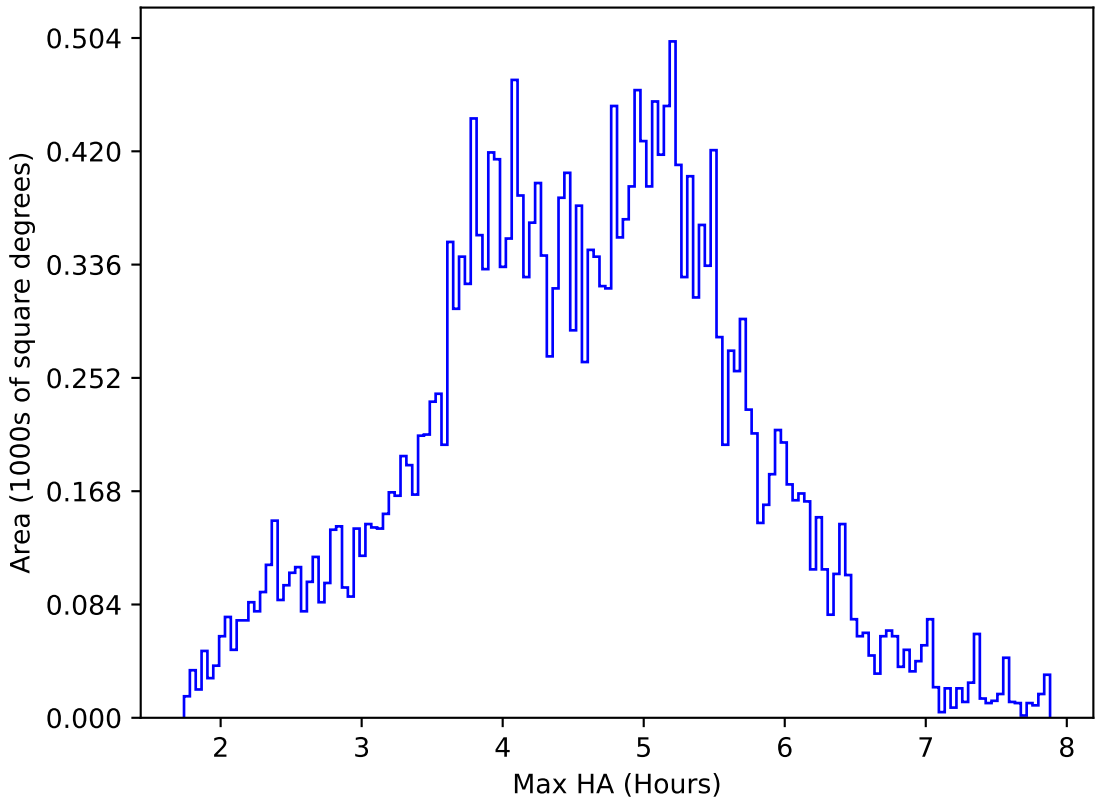
ddf_acor_sf15_lsf40_lsr20_v3.4_10yrs All sky i band: Max HA
