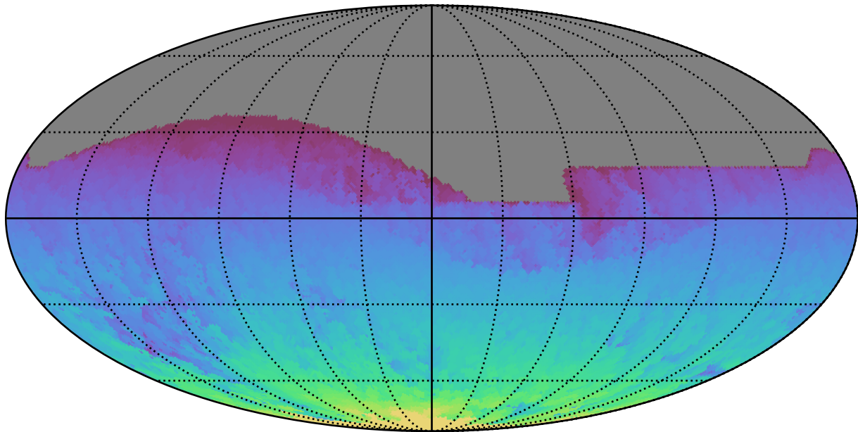
ddf_acor_sf15_lsf40_lsr20_v3.4_10yrs All sky all bands: Max HA
