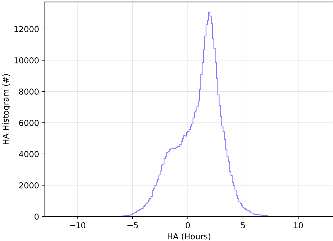
ddf_acor_sf15_lsf40_lsr20_v3.4_10yrs WFD y band: HA Histogram
