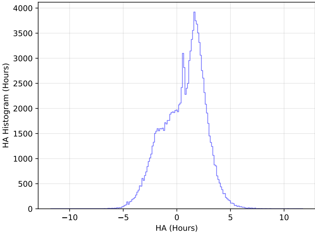
ddf_acor_sf15_lsf40_lsr20_v3.4_10yrs WFD u band: HA Histogram
