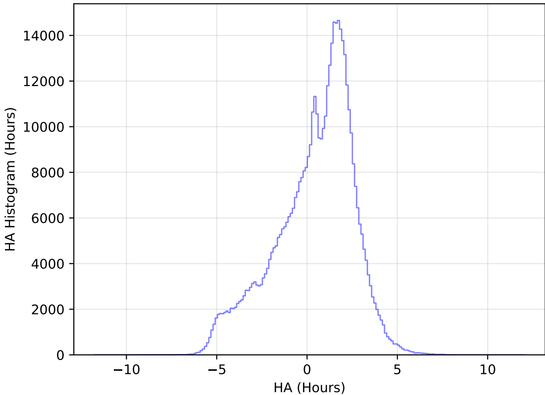
ddf_acor_sf15_lsf40_lsr20_v3.4_10yrs WFD r band: HA Histogram
