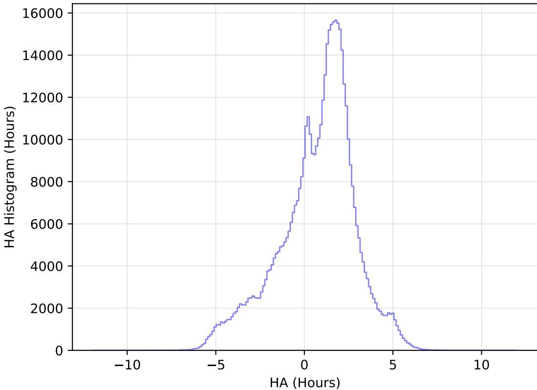
ddf_acor_sf15_lsf40_lsr20_v3.4_10yrs WFD i band: HA Histogram
