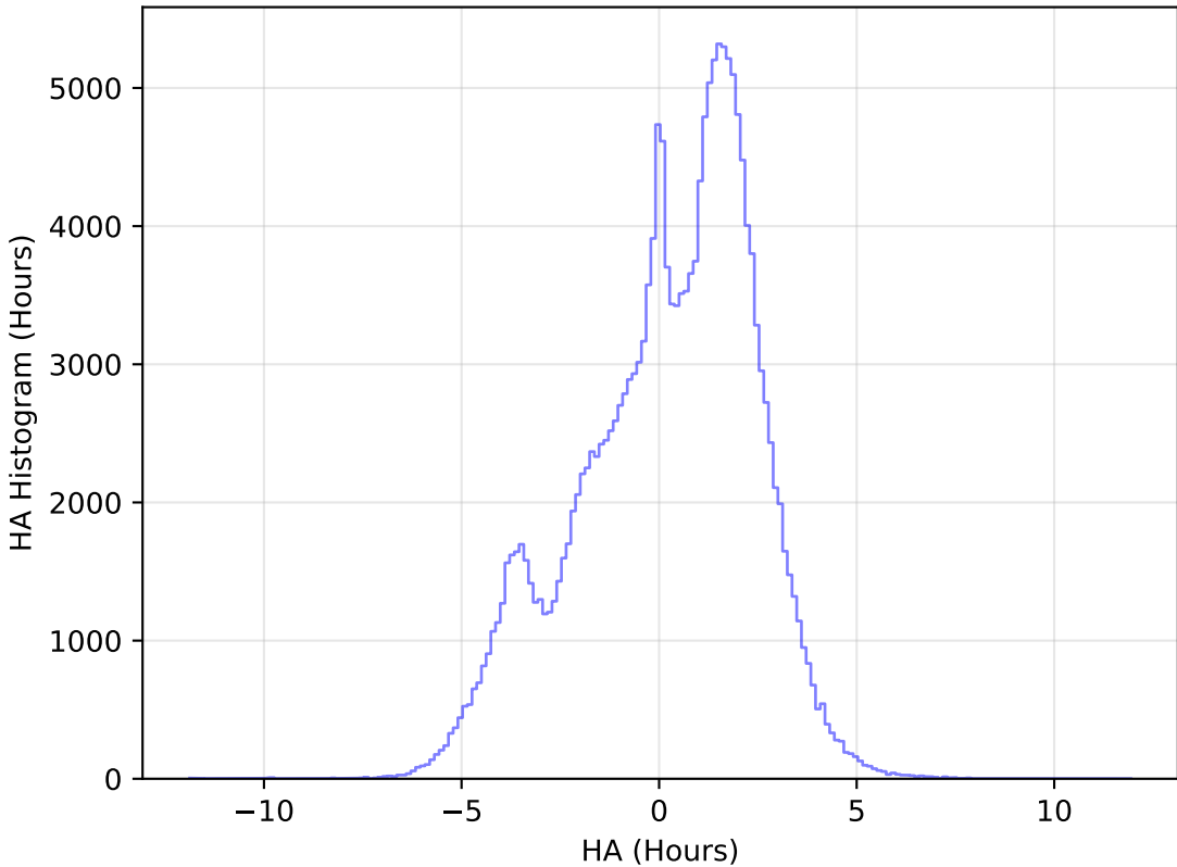
ddf_acor_sf15_lsf40_lsr20_v3.4_10yrs WFD g band: HA Histogram
