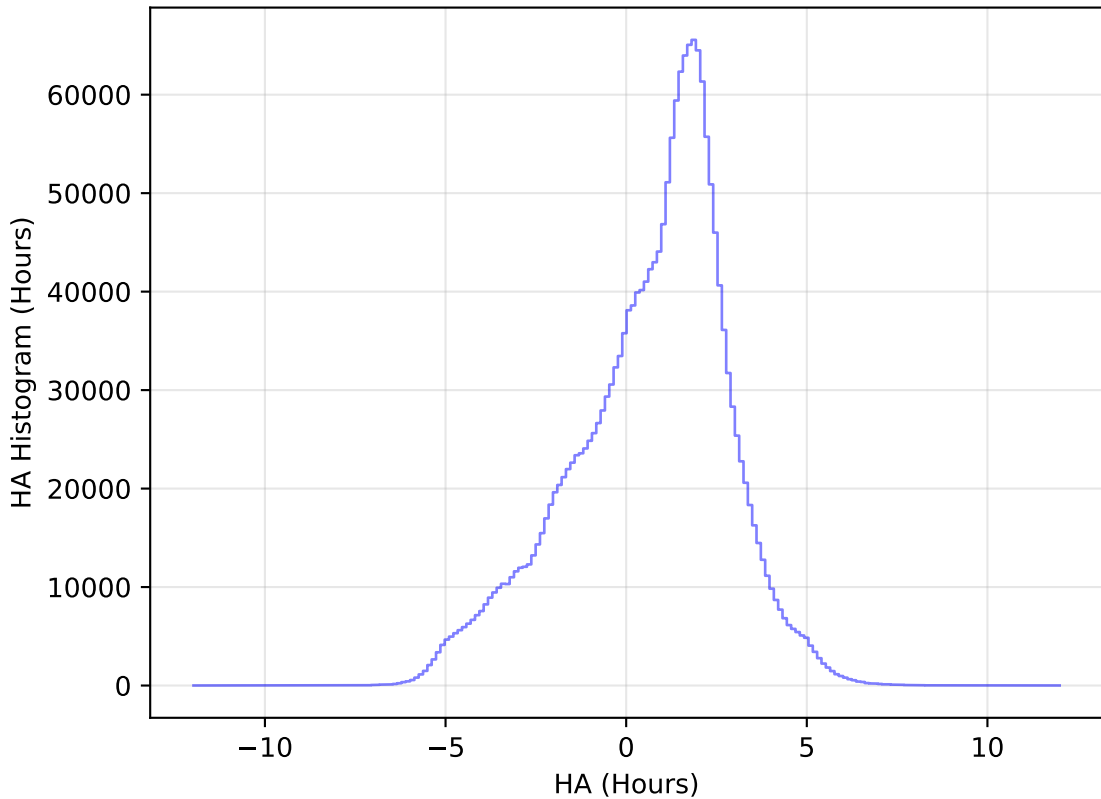
ddf_acor_sf15_lsf40_lsr20_v3.4_10yrs WFD all bands: HA Histogram
