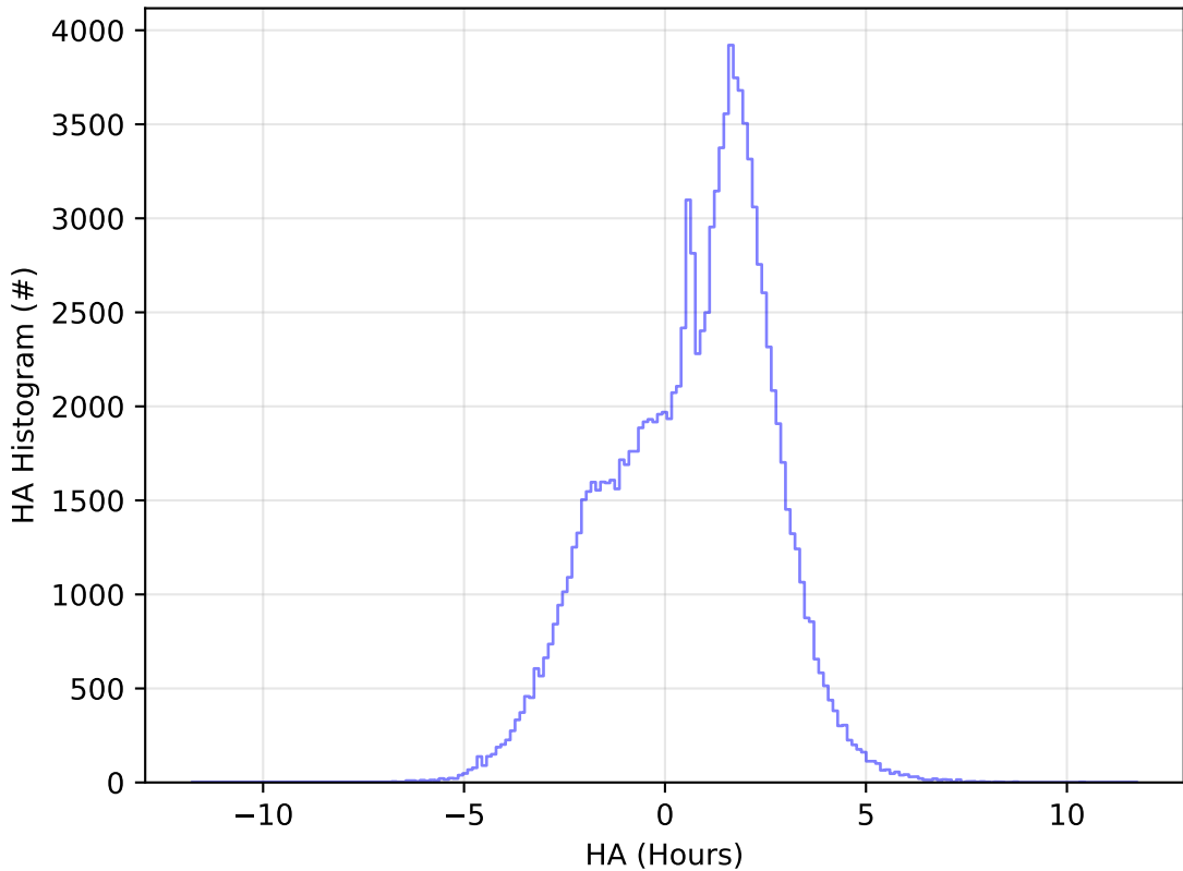
ddf_acor_sf15_lsf40_lsr20_v3.4_10yrs All sky u band: HA Histogram
