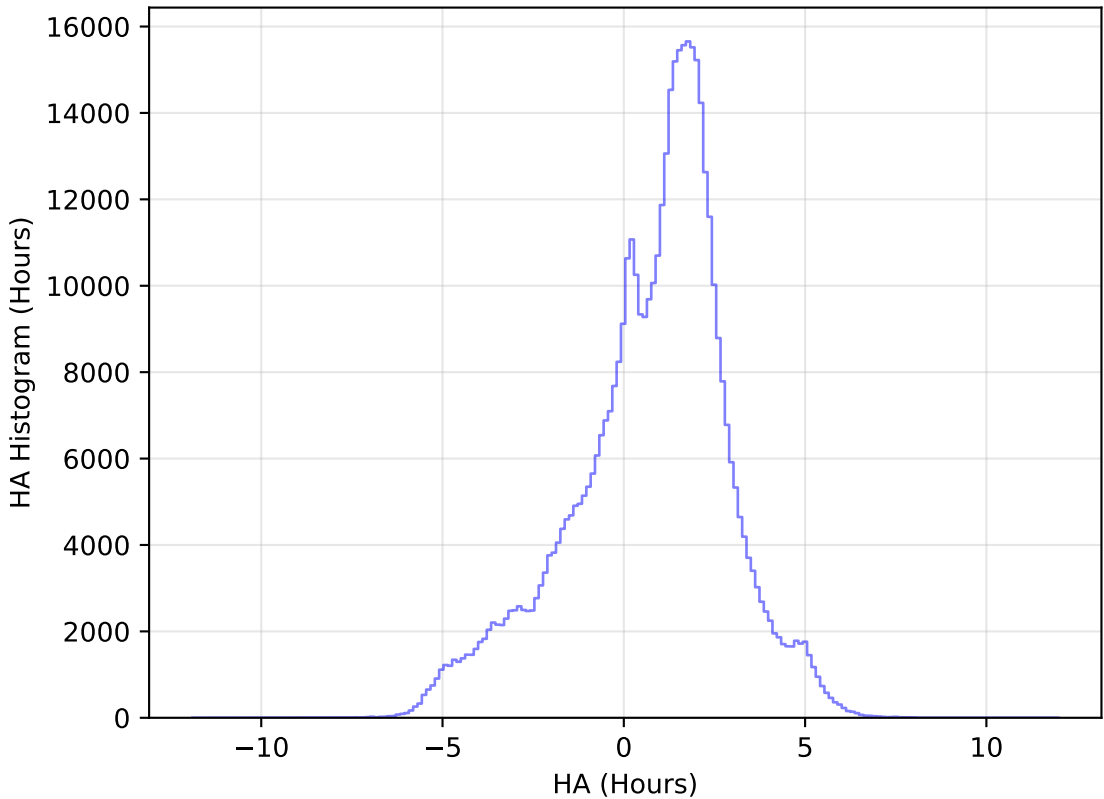
ddf_acor_sf15_lsf40_lsr20_v3.4_10yrs All sky i band: HA Histogram
