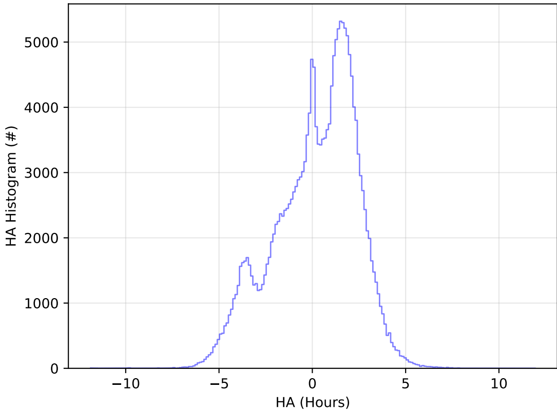
ddf_acor_sf15_lsf40_lsr20_v3.4_10yrs All sky g band: HA Histogram
