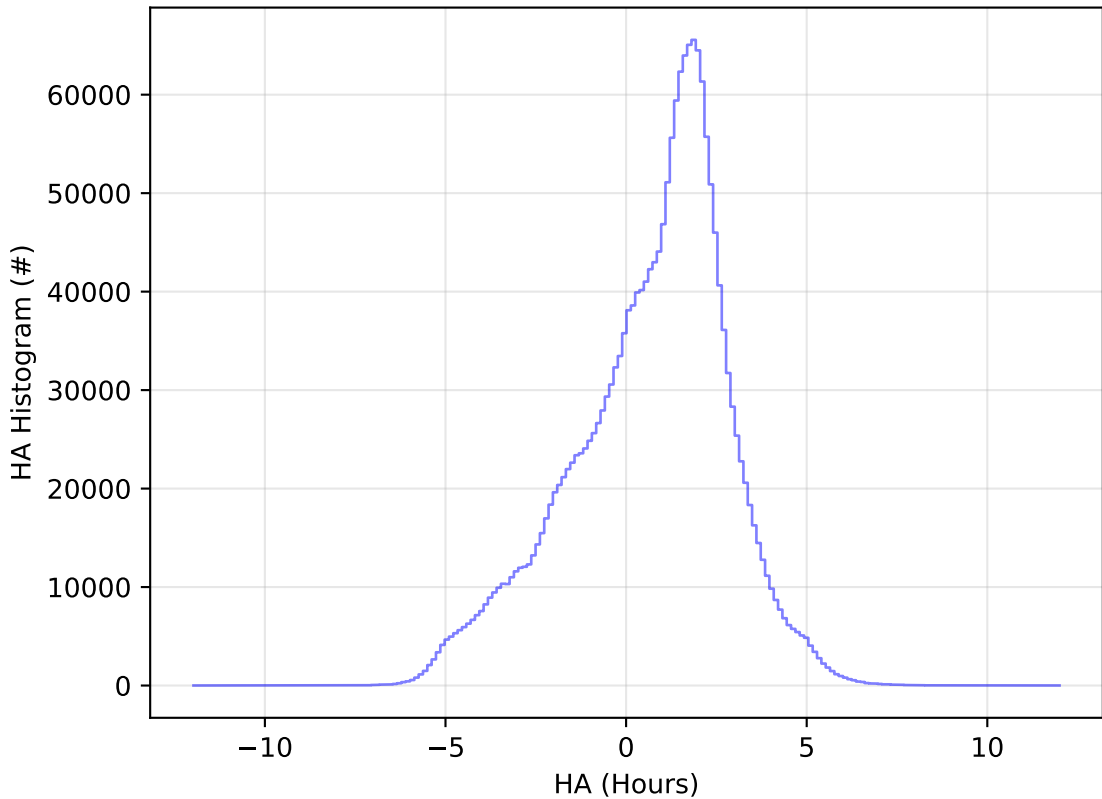
ddf_acor_sf15_lsf40_lsr20_v3.4_10yrs All sky all bands: HA Histogram
