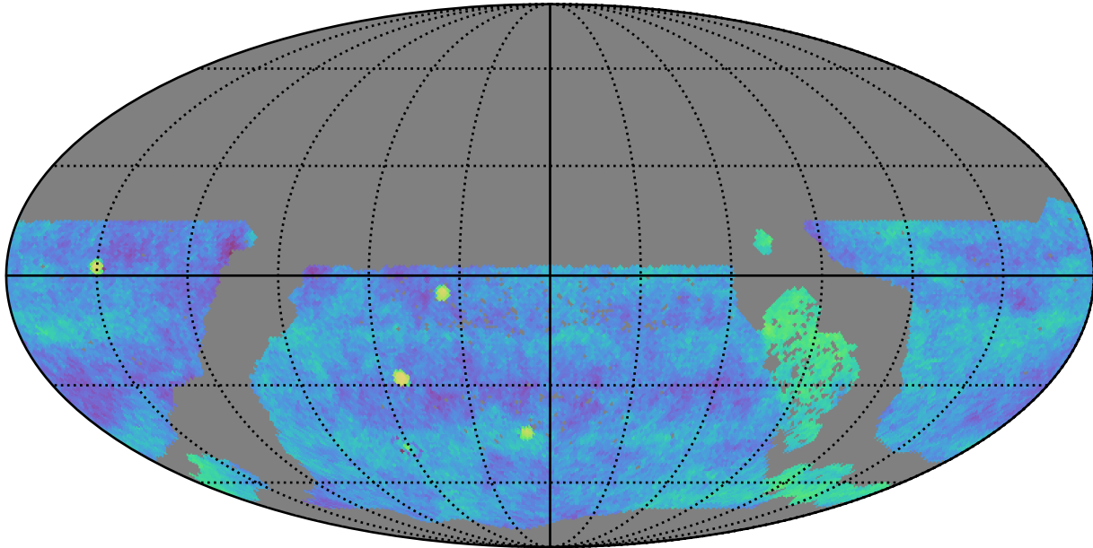
ddf_acor_sf15_lsf40_lsr20_v3.4_10yrs gri WFD: Fraction of visits in pairs (20-90 min)
