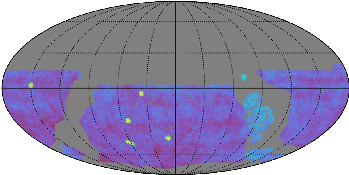
ddf_acor_sf15_lsf40_lsr20_v3.4_10yrs gri WFD: Fraction of visits in pairs (10-60 min)
